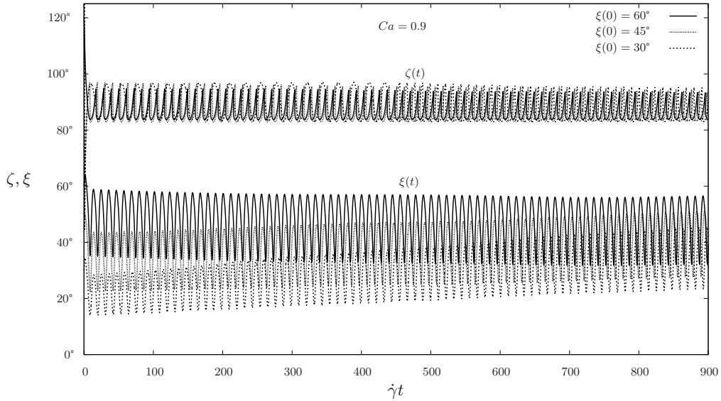
Figure 5: Wobbling motion for three initial orientations \xi(0) = 30^\circ, 45^\circ and 60^\circ at Ca = 0.9 ( \lambda = 1 ). The small axis oscillates a little about the shear plane, while A_3(t) precesses and oscillates around the vorticity axis with an inclination which tends to 44^\circ \pm 12^\circ for all three initial orientations.
