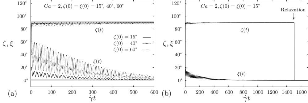
Figure 6: Time evolution of the angles \zeta(t) and \xi(t) at Ca = 2 ( \lambda = 1 ). (a) Time response ( \dot{\gamma}t \in [0, 600] ) of the capsule for different initial orientations showing the convergence towards a rolling motion; (b) Long time response (for \xi(0) = 15^\circ ) followed by a relaxation phase ( \mathbf{v}^\infty = 0 for \dot{\gamma}t \geq 1500 ), during which both \xi and \zeta go to zero, thus showing that the capsule revolution axis is aligned with the vorticity axis.
