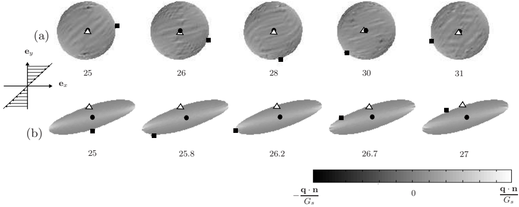
Figure 3: Capsule shape evolution over one half period at steady state when \zeta(0) = 0^\circ ( \lambda = 1 ): capsule in rolling regime. (a) Ca = 0.01 ( \max(\mathbf{q} \cdot \mathbf{n}/G_s) = 0.1 ); (b) Ca = 1.5 ( \max(\mathbf{q} \cdot \mathbf{n}/G_s) = 5 ). Same legend as in Figure 2. The points A_3(t) and M_3(t) are superimposed in (a), whereas A_3(t) is on the vorticity axis and M_3(t) is in the shear plane in (b).
