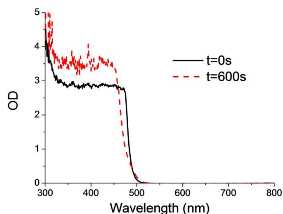
Fig. 12. Evolution of the UV-vis spectra of the curcumin derivative-coating after 600s of irradiation. Xe lamp, intensity = 30 \text{mW}/\text{cm}^2 . Formulation was sandwiched under 2 glass substrates.
