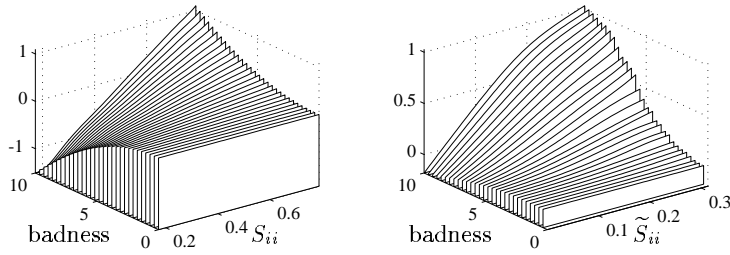
Figure 5. Maps of difference in prediction error PE - PE^{\text{bag}} vs. badness and leverage statistics, left: for ordinary least squares (all variables); right: for subset selection (one variable).
