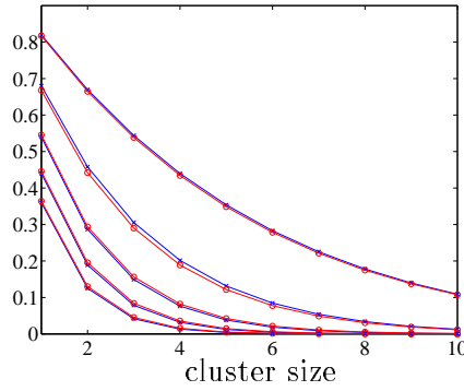
Figure 8. Probability of absence of a cluster vs. cluster size for subsampling with (o) and without (x) replacement for a training sample size of n = 50 . From top to bottom, subsample size is n' = 10, 20, 30, 40, 50 with replacement, and 9, 16, 23, 28, 32 \simeq n(1 - \exp(-n'/n)) without replacement.
