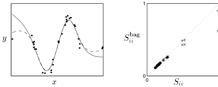
Figure 9. Left: pseudo-bagged cubic regression spline estimates for w^{b'} (dashed line) and w^{b''} (solid line); right: diagonal elements of the respective pseudo-bagged smoothing matrices S^{bag'} (+) and S^{bag''} (x) versus diagonal elements of the smoothing matrix S .
