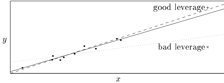
Figure 1. Least squares linear regression without the outlier in x (solid), with the good leverage point (dashed), and with the bad leverage point (dotted).
