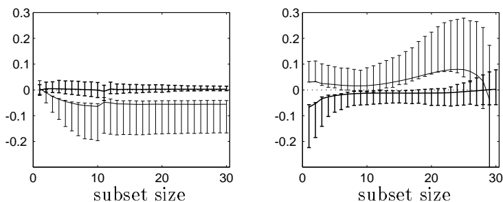
Figure 10. Average difference in prediction error between bagged regressors obtained by sampling with and without replacement vs. number of selected variables. A proportion P is sampled with replacement, and a proportion P/(P+1) (thin line), or 1 - \exp(-P) (bold line) is sampled without replacement. The bars cover 90% of the distributions of differences. Left: P = 0.2 , right: P = 1 .
